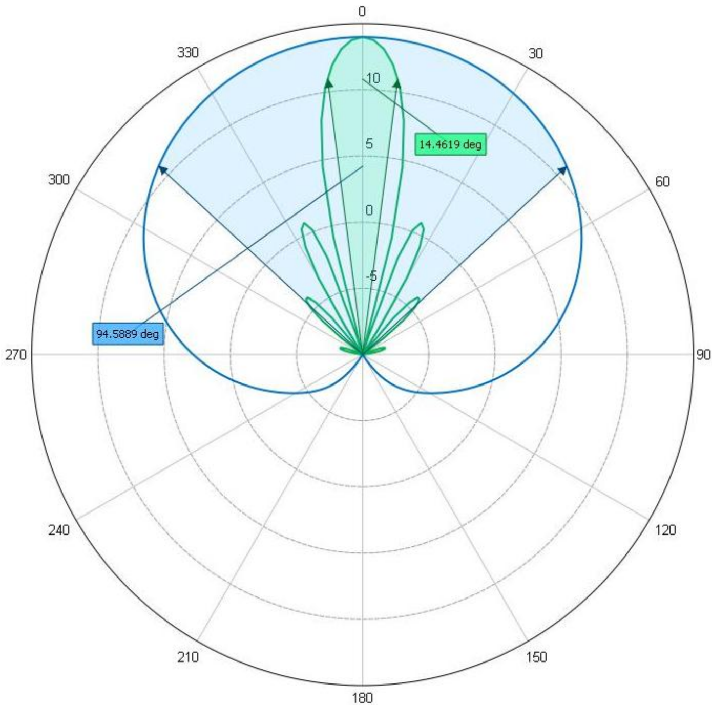
Azimuth Pattern
