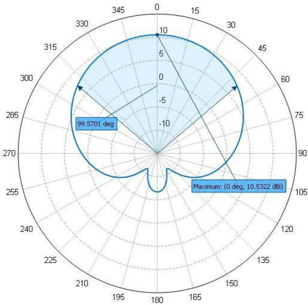
Azimuth Pattern
