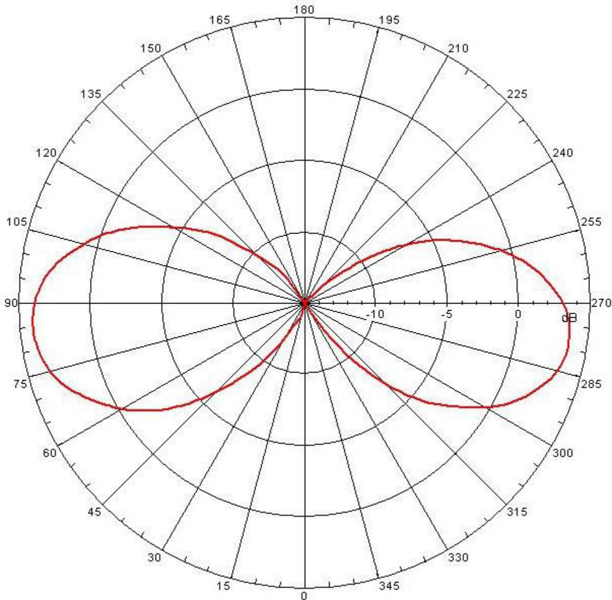
Elevation Pattern
