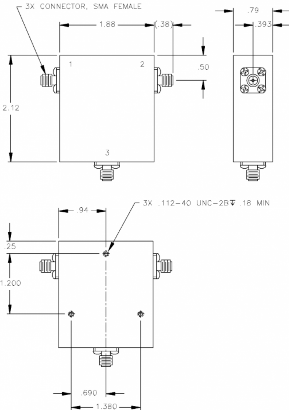
Engineering Drawing
