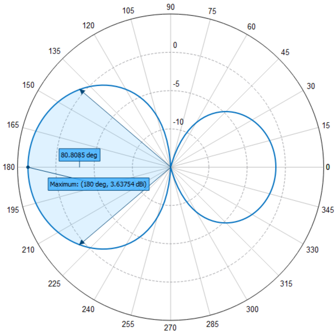
Elevation Pattern
