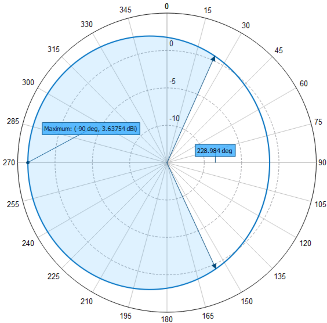
Azimuth Pattern
