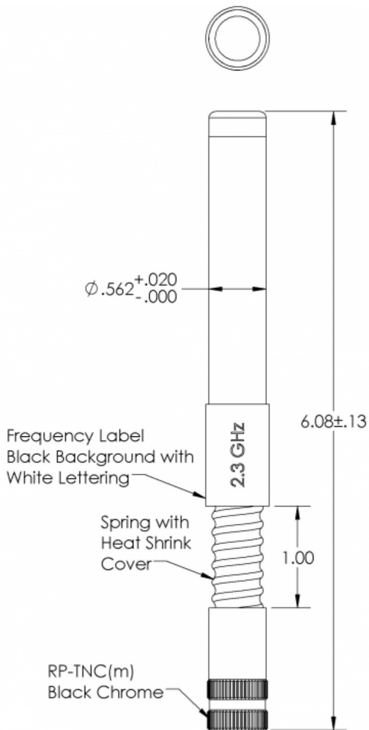
Engineering Drawing
